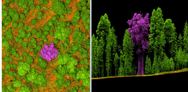
Figure 1. Fixed wing lidar and imagery data from the Sequoia National Forest images the 'General Sherman' tree and yields quantitative estimates of fuel loads in the canopy and on the forest floor.
